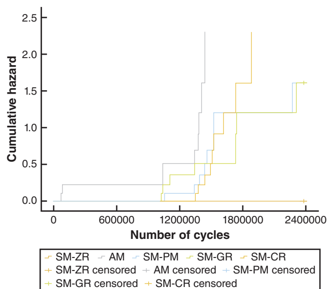
Figure 5. Cumulative hazard curves of tested materials after cyclic loading. AM, additively manufactured interim resin; SM-CR, high-impact polymer composite resin; SM-GR, graphene-reinforced polymethyl methacrylate; SM-PM, polymethyl methacrylate; SM-ZR, strength gradient zirconia.
