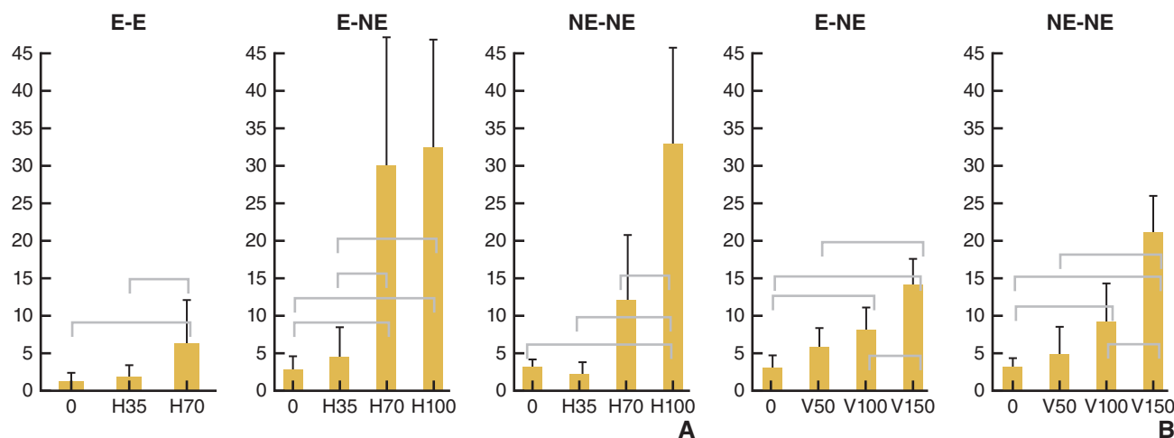
Figure 4. Mean values represent difference in MGX measurements in passive fit and active fit situations for different abutment-type combination groups with different misfit levels. Brackets indicate statistically significant differences ( P < .05 ) between groups (1-way ANOVA).
