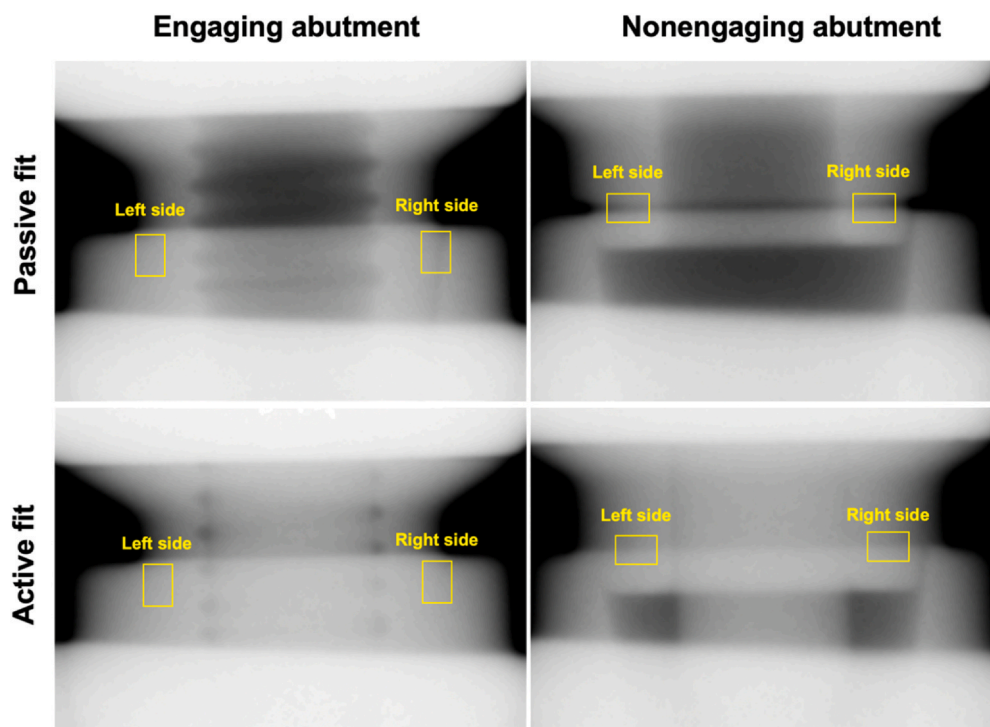
Figure 3. MGX measurements of H70 misfit group on side B implant during passive fit and active fit for engaging (left side) and nonengaging (right side) abutments.
